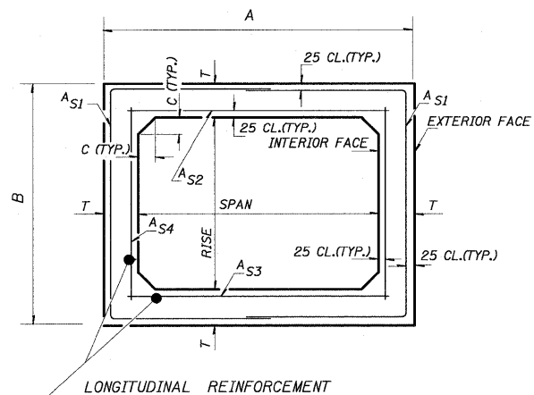
CROSS SECTION
