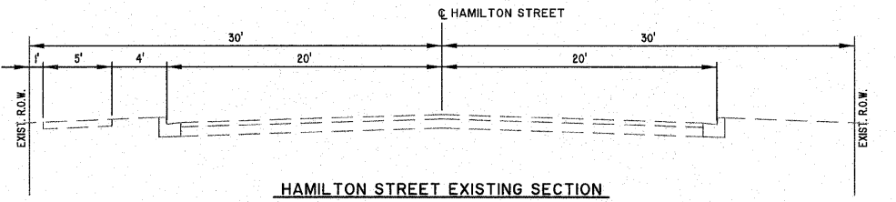
HAMILTON STREET EXISTING SECTION JACKSON STREET TO SCOTT STREET STATION 110+00.00 TO STATION 112+16.12
