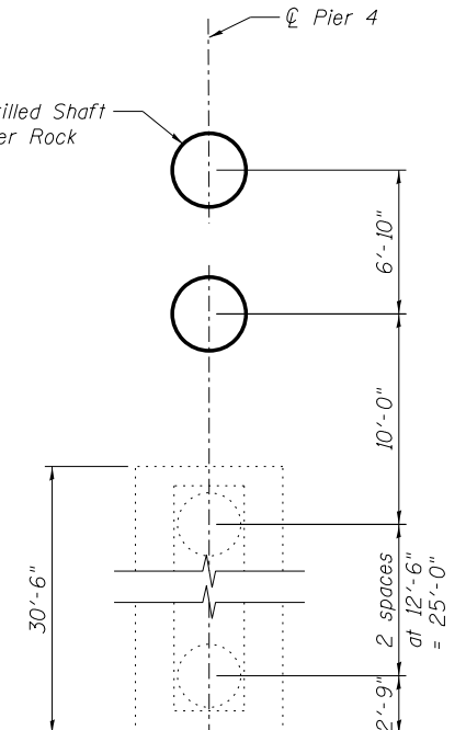
PIER 4 FOUNDATION PLAN
