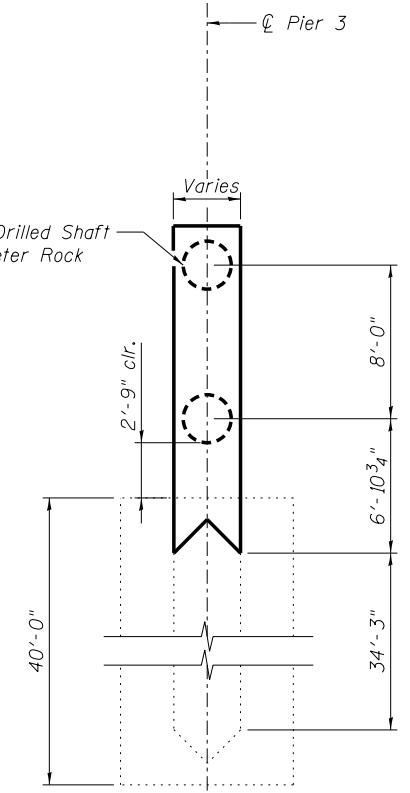
PIER 3 FOUNDATION PLAN
