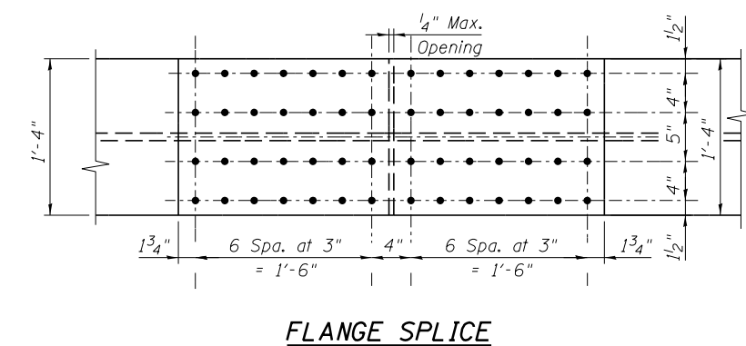
FIELD SPLICE #2 (Girders 1-3)
