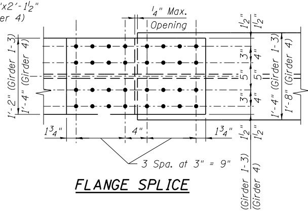
FIELD SPLICE #1 (Girders 1-4)
