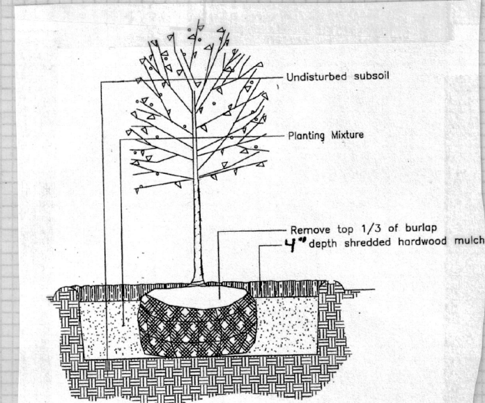
Detail Deciduous Tree Planting
