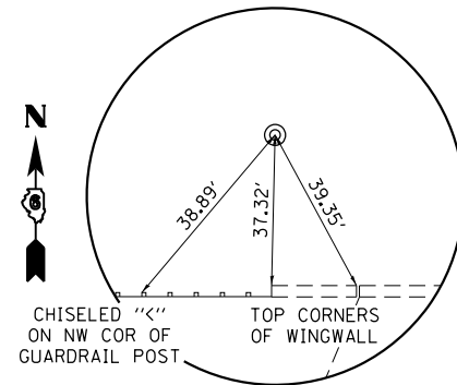
POT STA 534+00.86 PSM 9900 DISC IN CONCRETE
