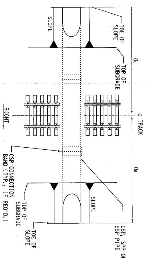
PLAN - SINGLE TRACK SCALE: NONE
