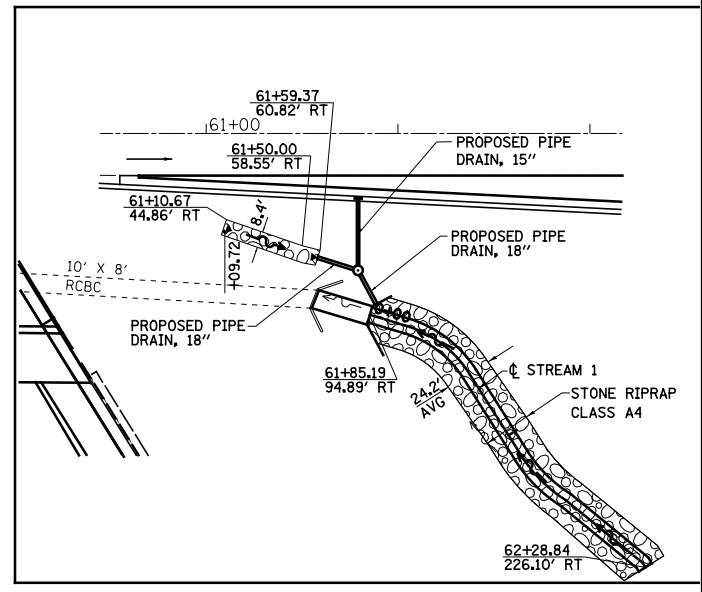
DETAIL (RAMP A INFIELD)
