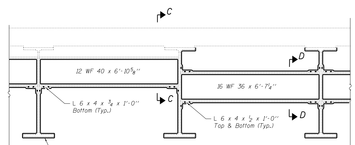
Limits of application for Cleaning and Painting Steel Bridge SECTION A-A SHOWING DIAPHRAGM D1 SHOWING DIAPHRAGM D2 SECTION B-B Limits of application for Cleaning and Painting Steel Beams (Typ.) SECTION C-C Limits of application for Cleaning and Painting Steel Bridge SECTION D-D
