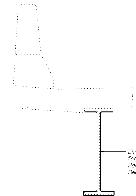
Limits of application for Cleaning and Painting Steel Bridge SECTION A-A SHOWING DIAPHRAGM D1 SHOWING DIAPHRAGM D2 SECTION B-B Limits of application for Cleaning and Painting Steel Beams (Typ.) SECTION C-C Limits of application for Cleaning and Painting Steel Bridge SECTION D-D
