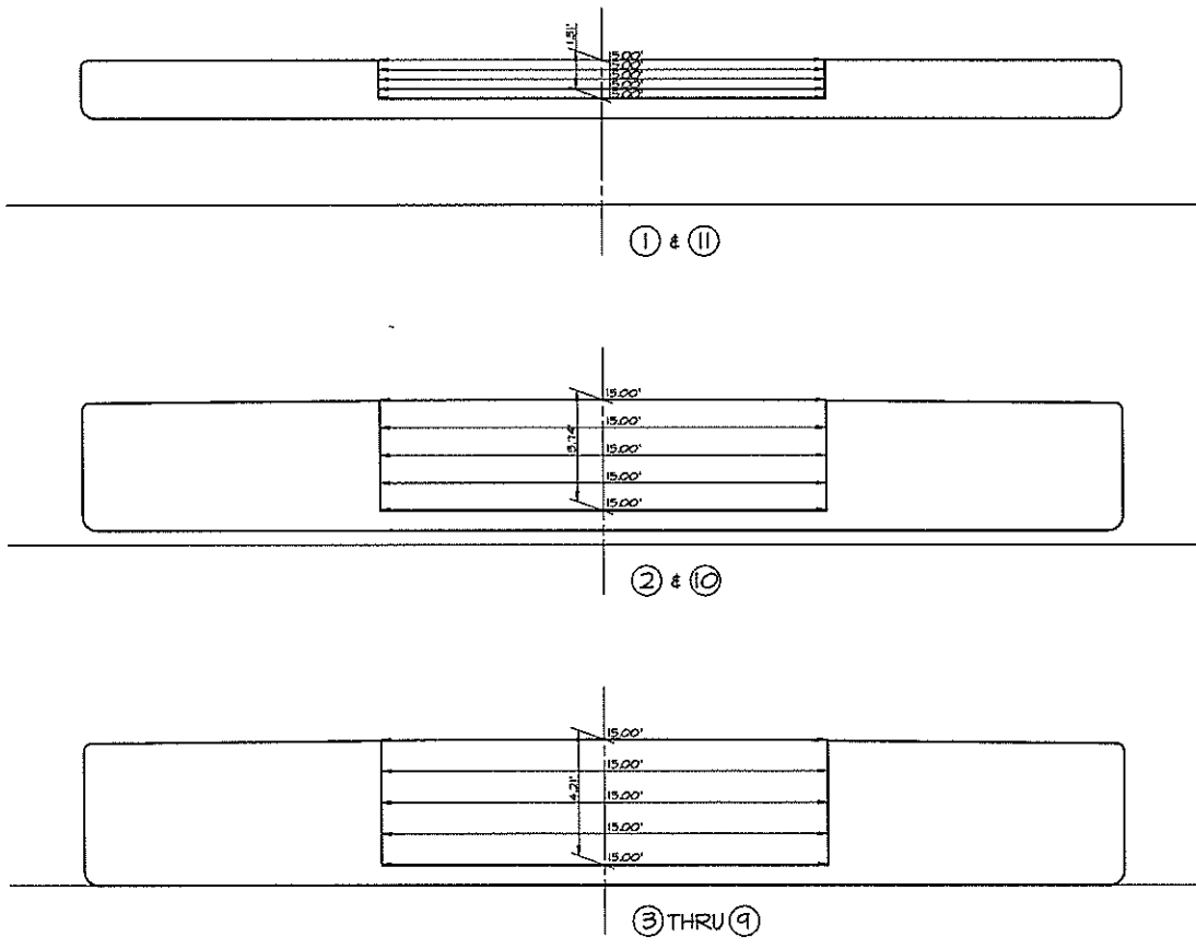
TONNAGE SECTIONS SCALE 3/8" = 1'-0"
