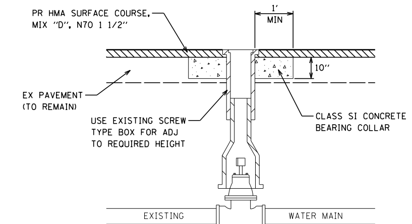
VALVE BOX FRAME TO BE ADJUSTED DETAIL NOT TO SCALE
