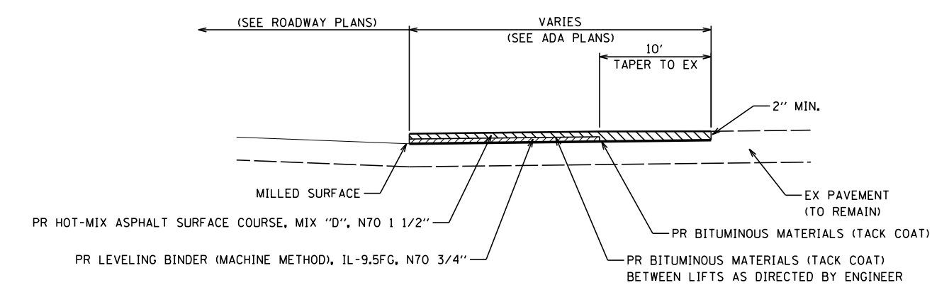
SIDE ROAD TYPICAL SECTION DETAIL NOT TO SCALE
