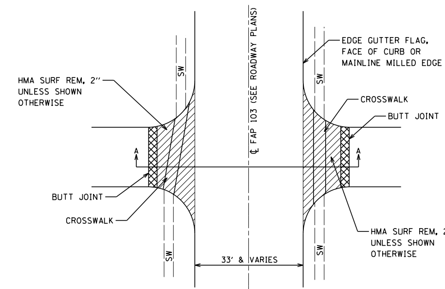
SIDE ROAD MILLING AND BUTT JOINT DETAIL NOT TO SCALE
