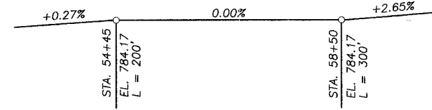
GRADE PROFILE
