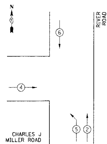
TEMPORARY PHASE DESIGNATION DIAGRAM
