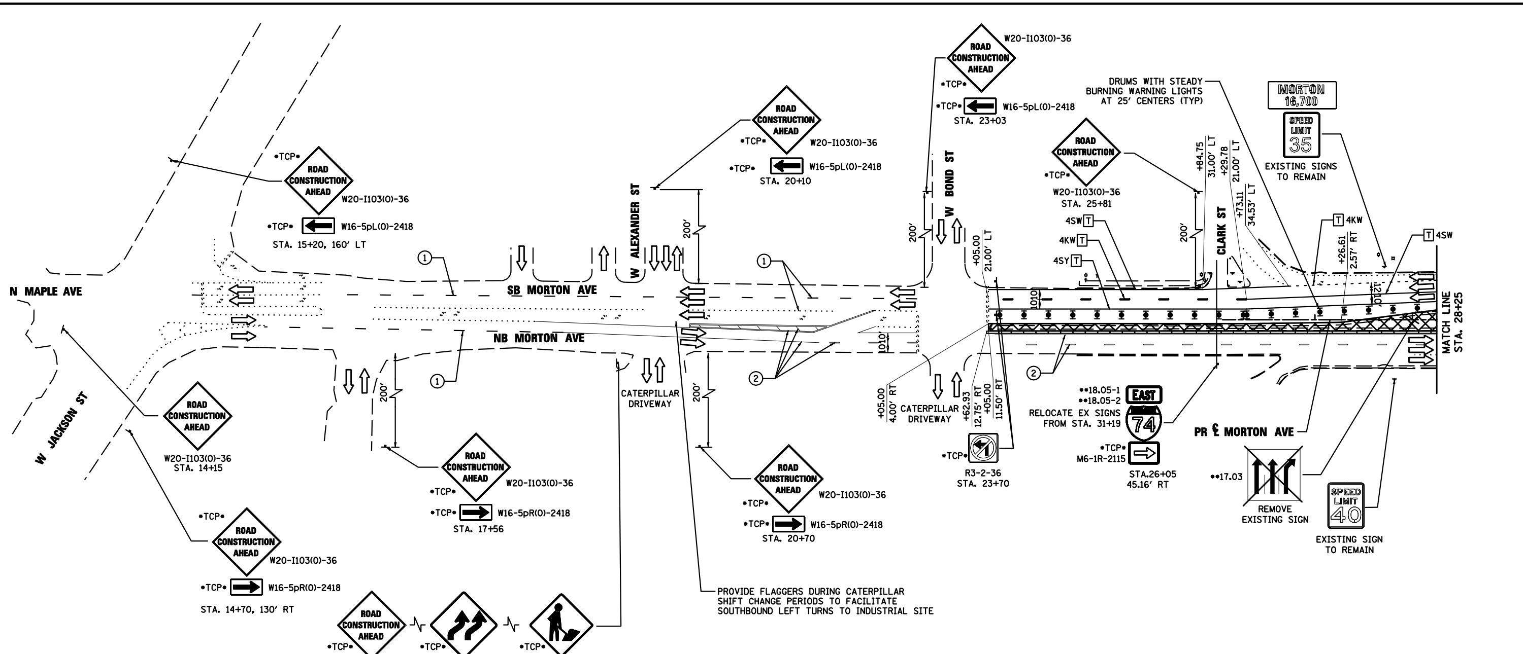
NORTH BOUND MORTON AVENUE APPROACH SIGNING DETAIL
