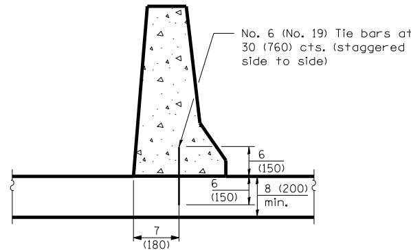
NEW OR EXISTING PCC BASE
