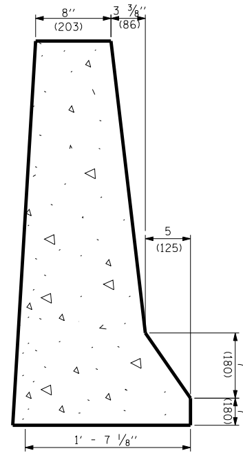
TYPICAL CROSS-SECTION
