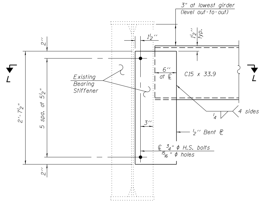
END DIAPHRAGM - D1 (Looking Upstation)
