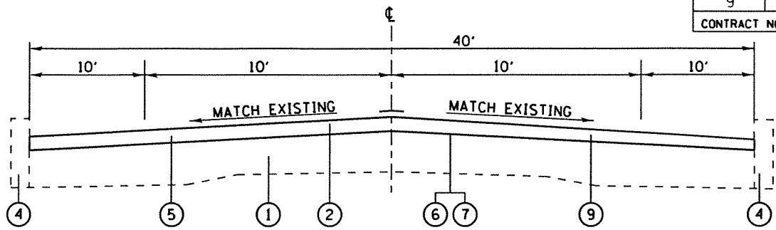
26TH - 29TH TYPICAL SECTION STA 0+00 TO STA 7+32
