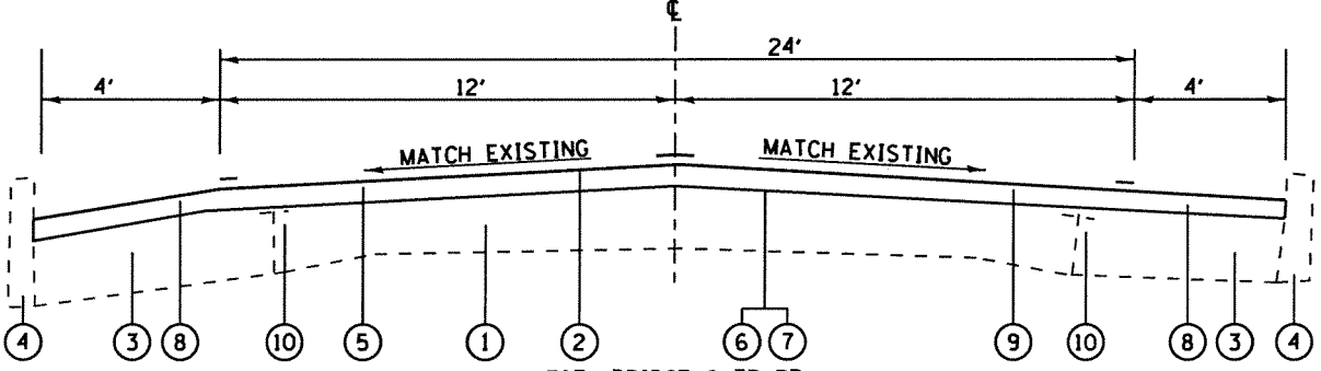
36TH-BRIDGE OVER RR TYPICAL SECTION STA 33+95 TO STA 54+90
