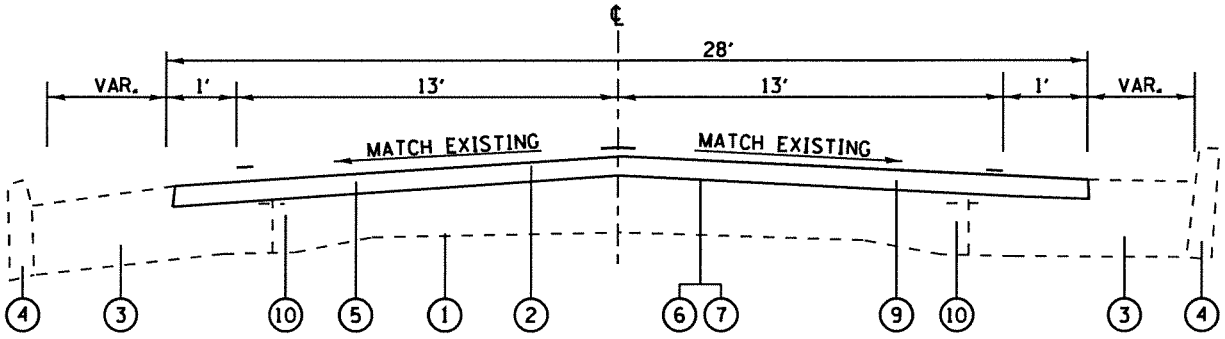
29TH - 36TH TYPICAL SECTION STA 7+32 TO STA 7+95 (OMISSION) STA 7+95 TO STA 33+95
