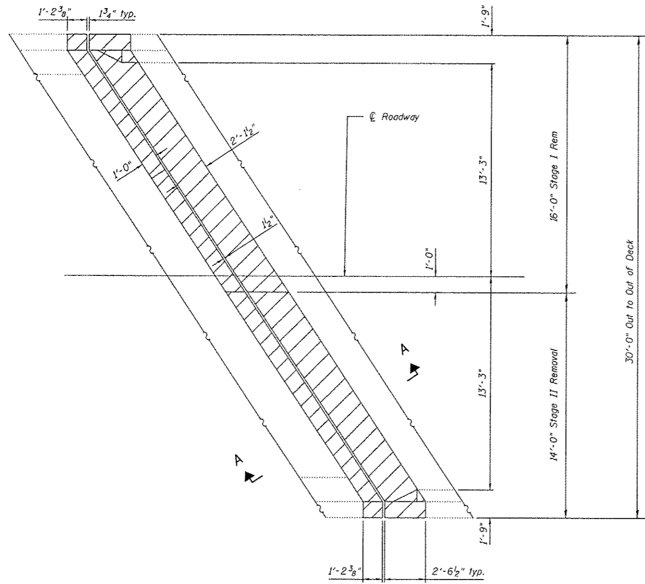
CONCRETE REMOVAL (W. Abutment)
