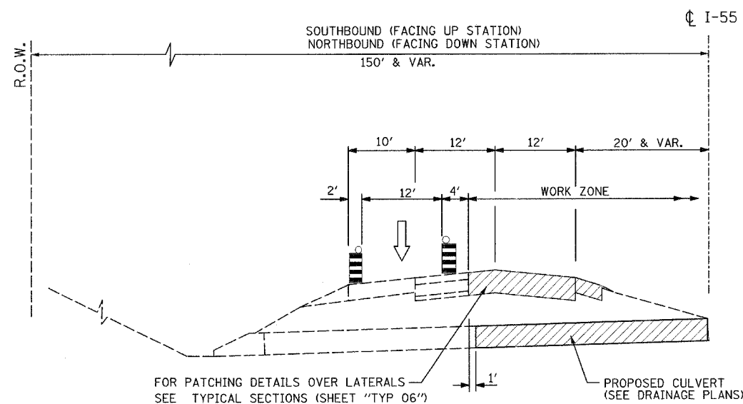
PRE-STAGE, PHASE II STORM SEWER LATERALS CONSTRUCTION
