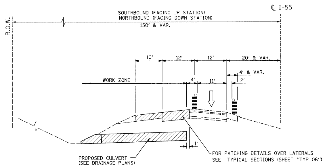
PRE-STAGE, PHASE I STORM SEWER LATERALS CONSTRUCTION
