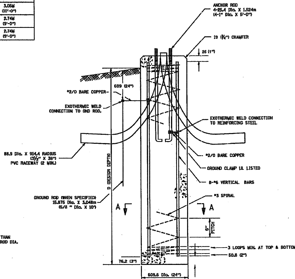
FOUNDATION DETAIL
