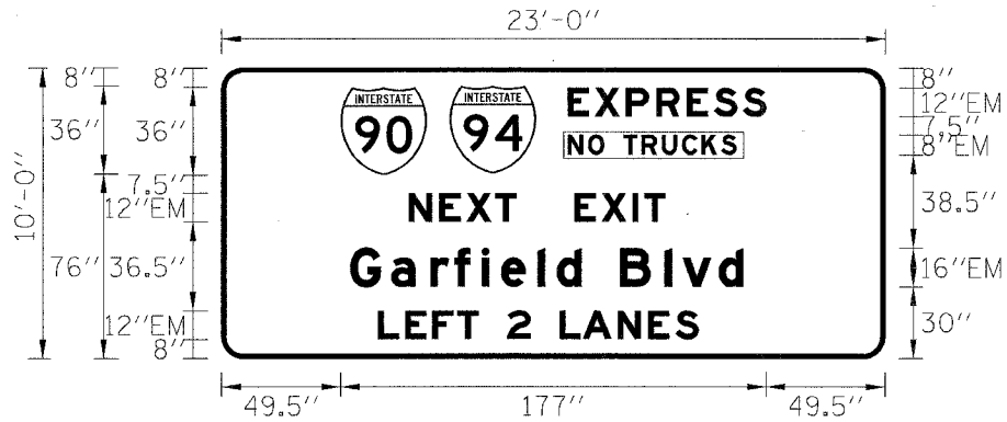
SIGN DETAIL 1:100
