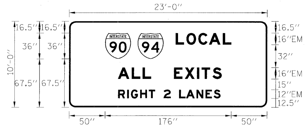
SIGN DETAIL 1:100
