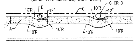
IMMOVABLE OBJECTS (SIDEWALK WITH PARKWAY)
