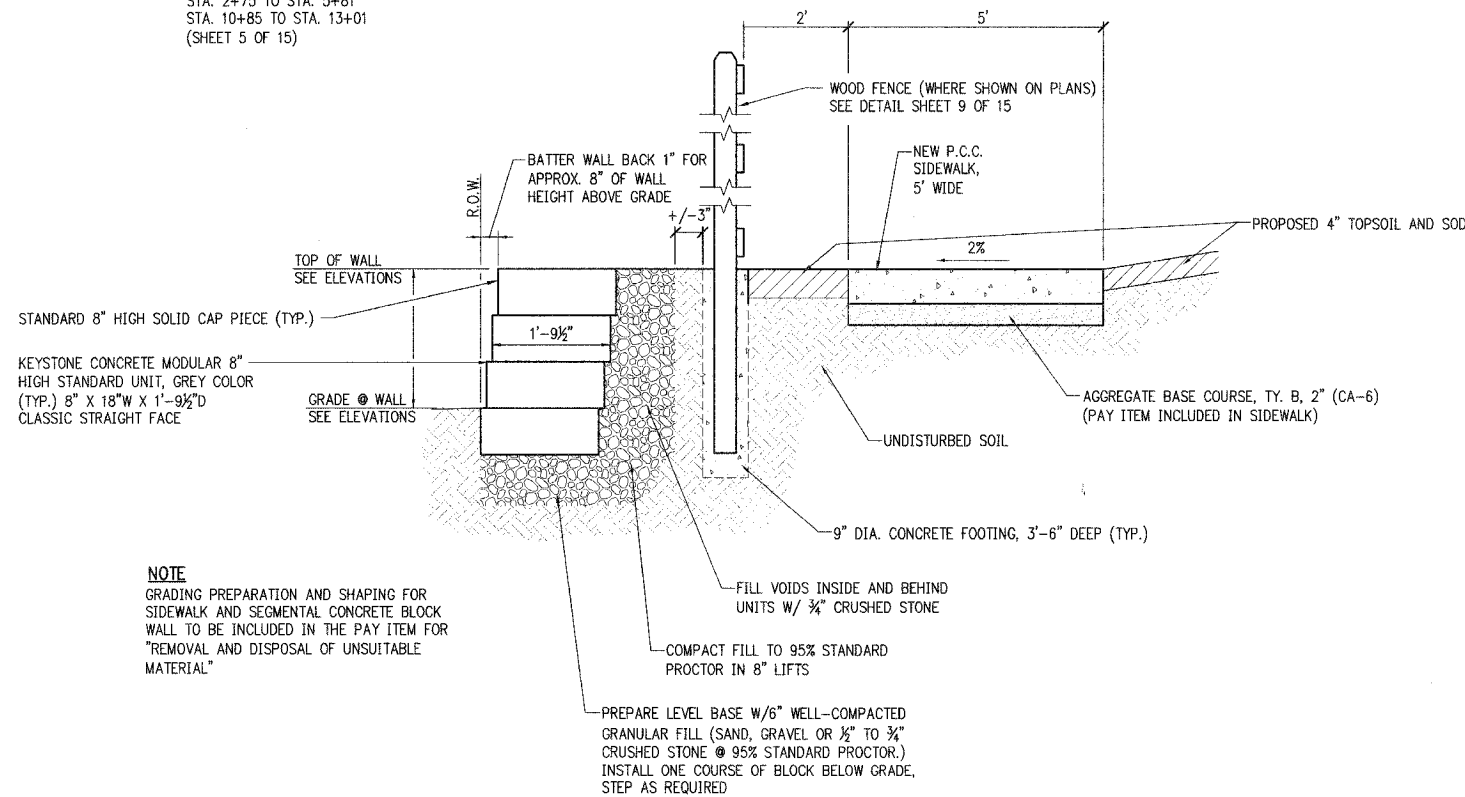
SEGMENTAL CONCRETE BLOCK WALL TYPICAL SECTION
