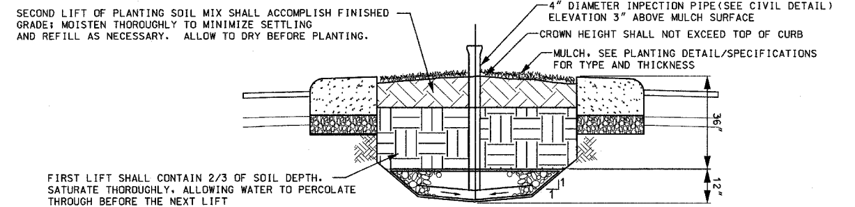
SOIL DETAIL NTS
