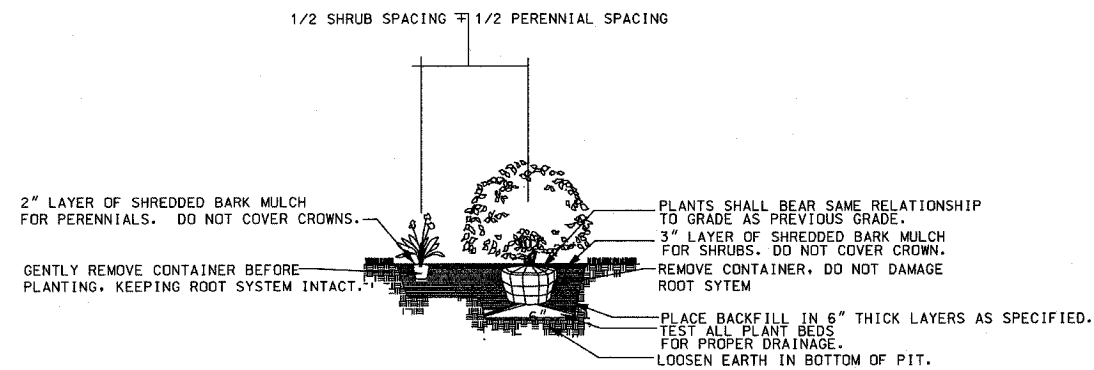
SHRUB AND PERENNIAL PLANTING DETAIL NTS
