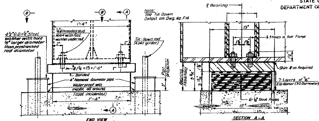
ELASTOMERIC BEARING AT ABUTMENT REAR WALL (TYPE I)
