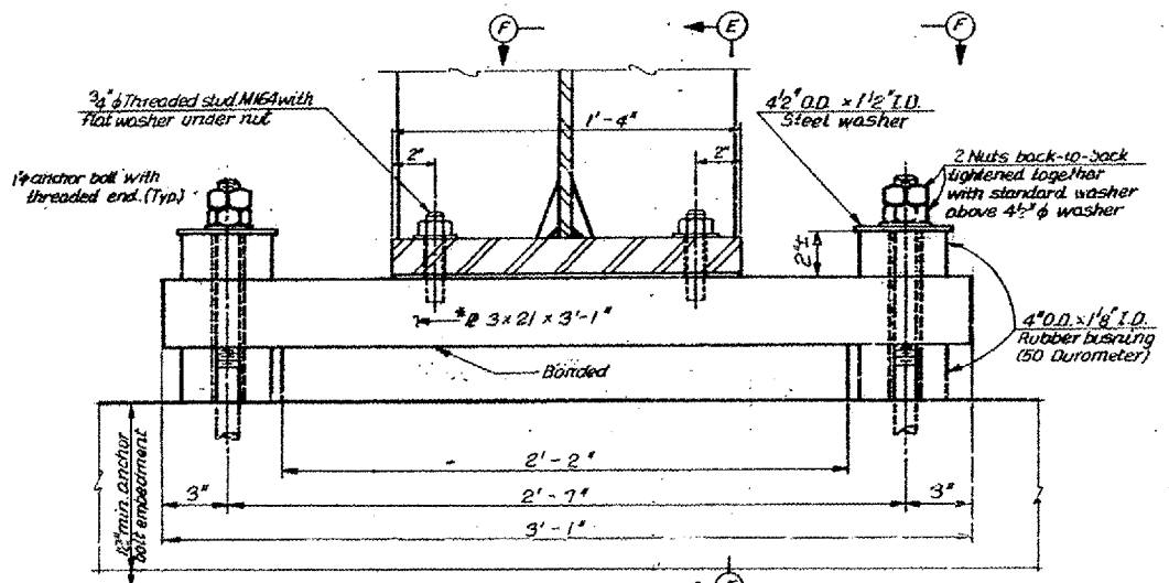
ELASTOMERIC BEARING AT ABUTMENT FRONT WALL (TYPE I)
