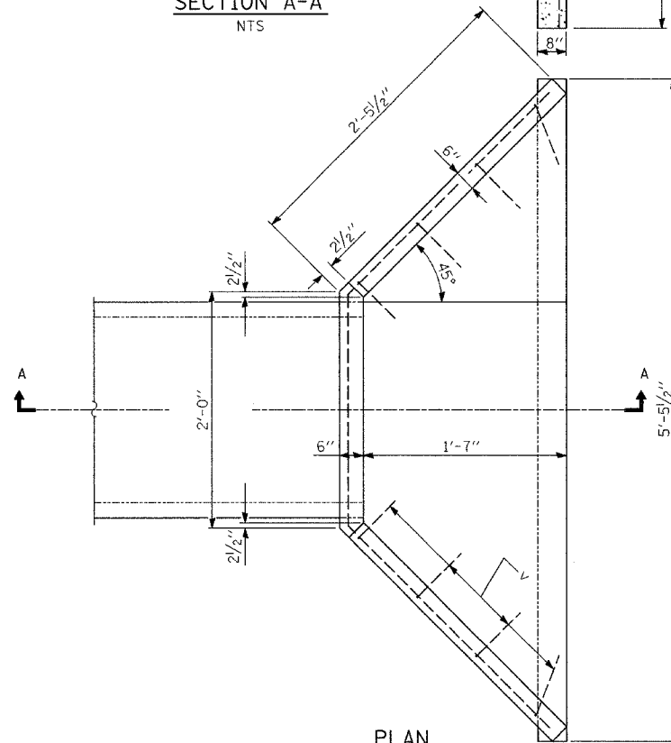
PLAN NTS
