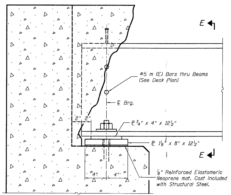
BEARING DETAIL Not to Scale
