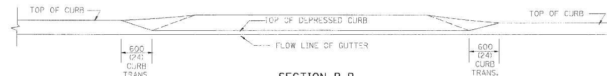
SECTION B-B
