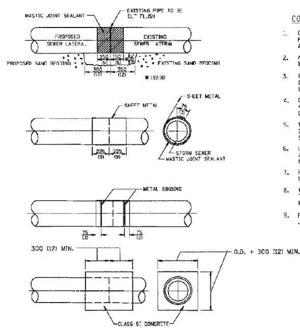
DETAIL "B" CLASS SI CONCRETE COLLAR
