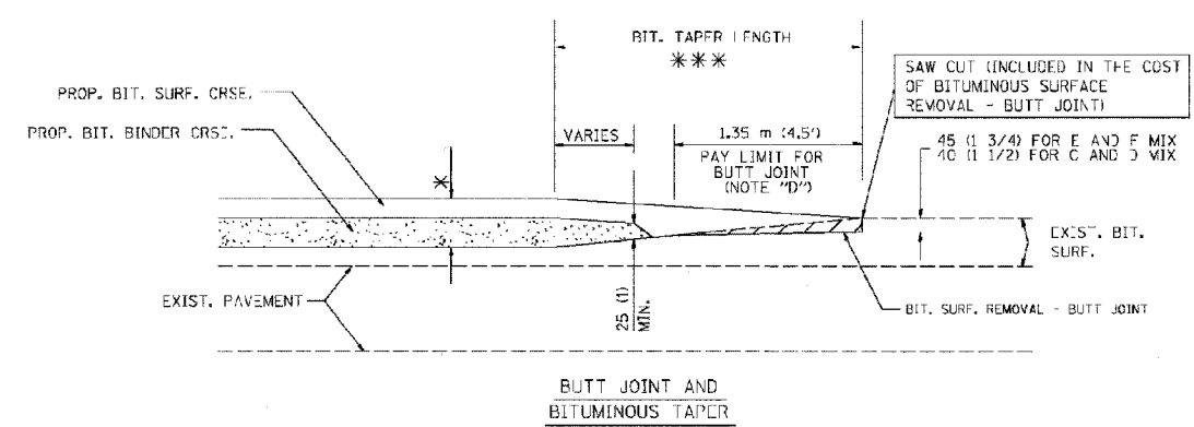
OPTION 2 TYPICAL TEMPORARY RAMP
