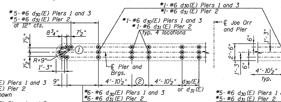
DOWEL LAYOUT
