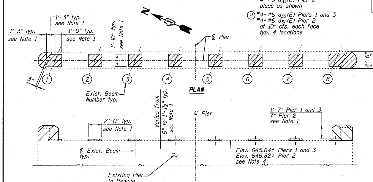
REMOVAL SKETCH
