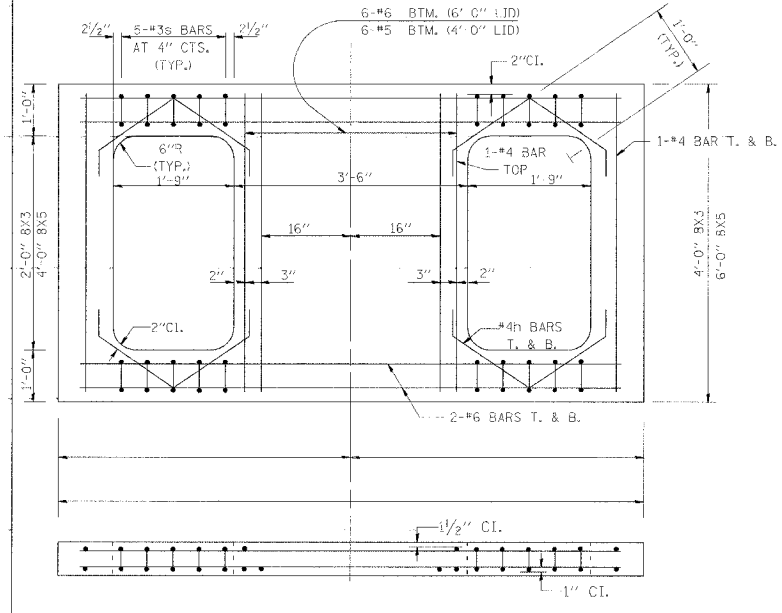
REINFORCED LID FOR TYPE 20 & 22 FRAME & GRATE
