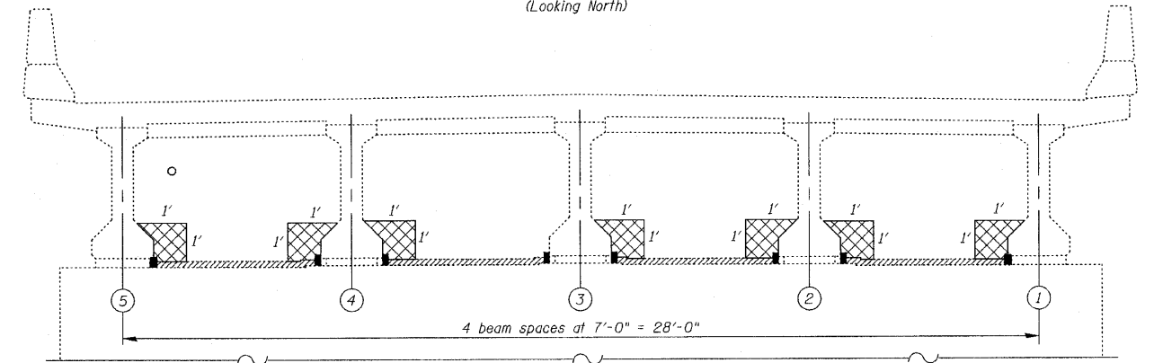
DIAPHRAGM AT FIXED PIER #2 (Looking North)
