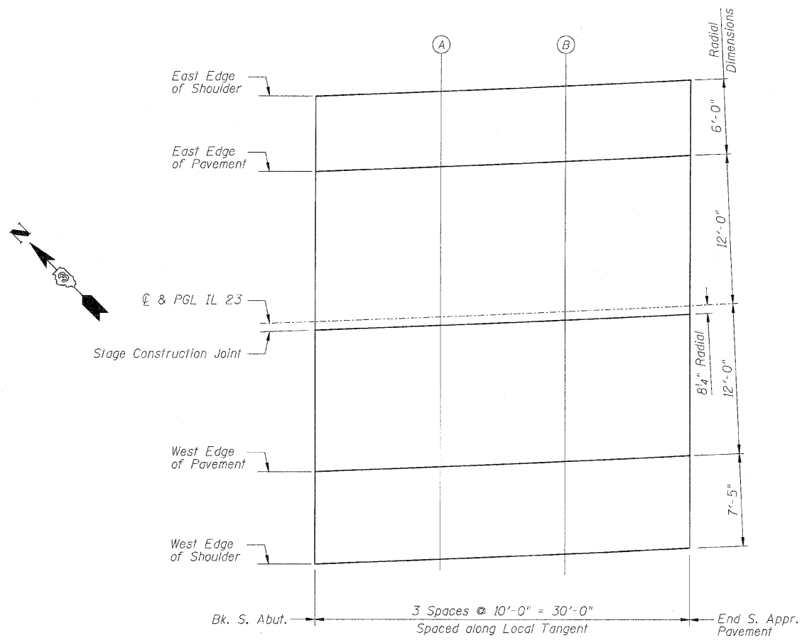
PLAN FOR TOP OF SLAB ELEVATIONS
