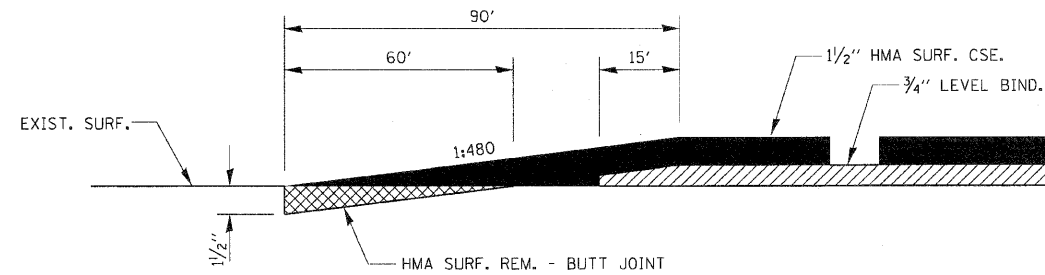
BUTT JOINT DETAIL 406-9
