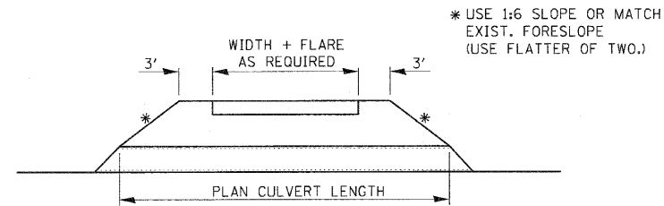
FIELD ENTRANCE DETAIL 402-1
