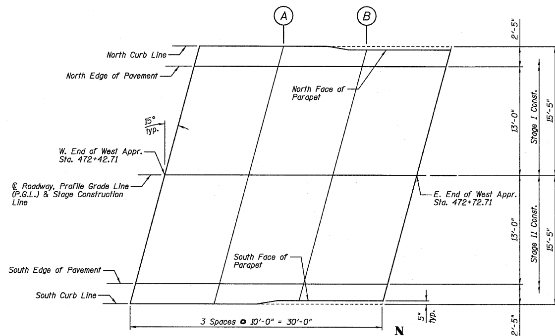
WEST APPROACH SLAB PLAN
