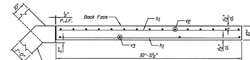
UPPER WINGWALL PLAN
