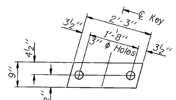
FABRIC BEARING PAD (Interior) (12 Required)
