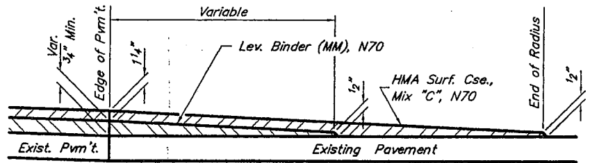
SECTION A-A SIDE ROAD (Est. No. = 8)
