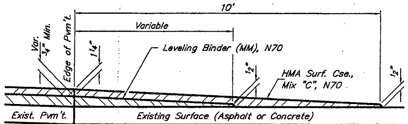
SECTION A-A PRIVATE ENTRANCE - ASPHALT (Est. No. = 1)
