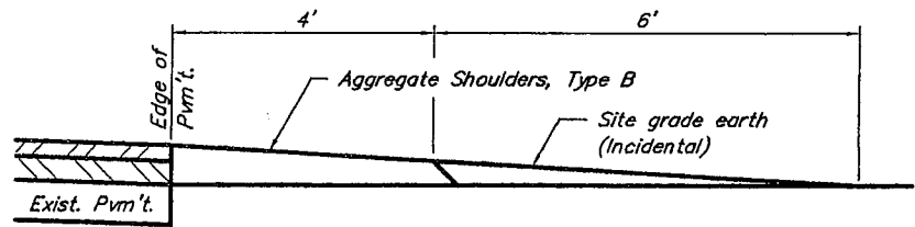
SECTION A-A FIELD ENTRANCE (Est. No. = 10)
