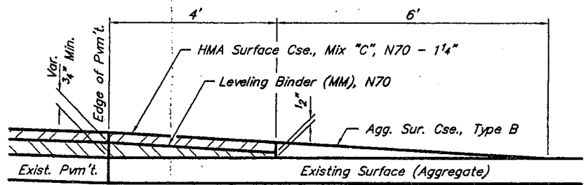
SECTION A-A PRIVATE ENTRANCE - AGGREGATE (Est. No. = 41)
