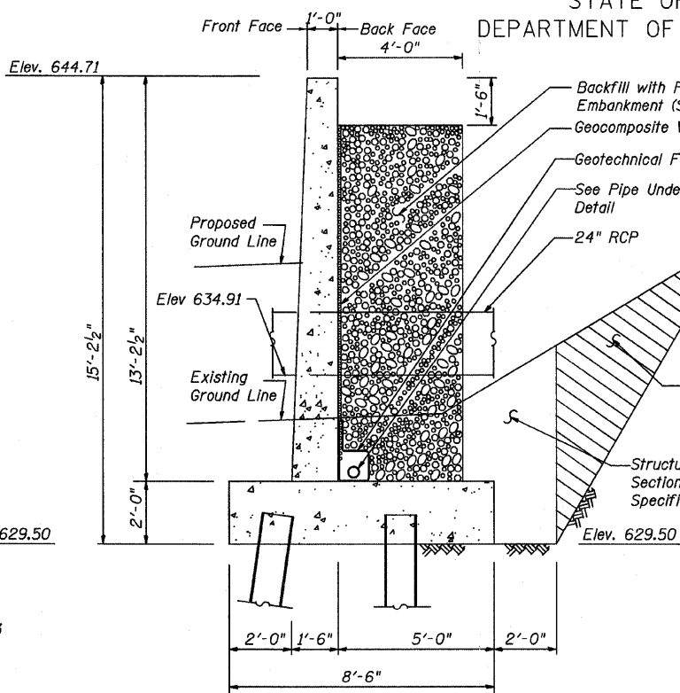
SECTION SHOWING DRAINAGE
