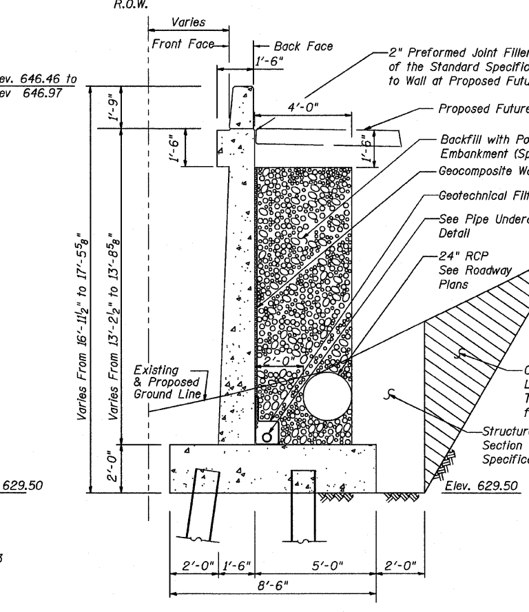
SECTION SHOWING DRAINAGE
