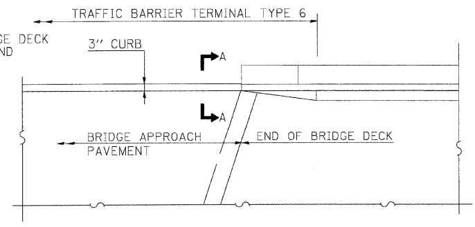
PARAPET TO CURB TRANSITION INTEGRAL ABUTMENT
