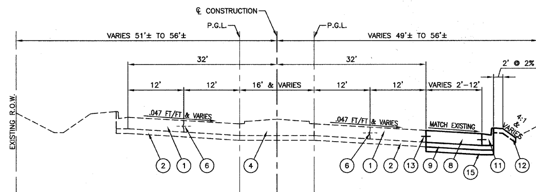
PROPOSED TYPICAL CROSS SECTION HARLEM AVENUE STA. 116+00 TO STA. 119+80
