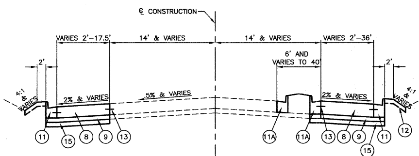
PROPOSED TYPICAL CROSS SECTION ACCESS ROAD WEST OF HARLEM AVENUE LOOKING EAST
