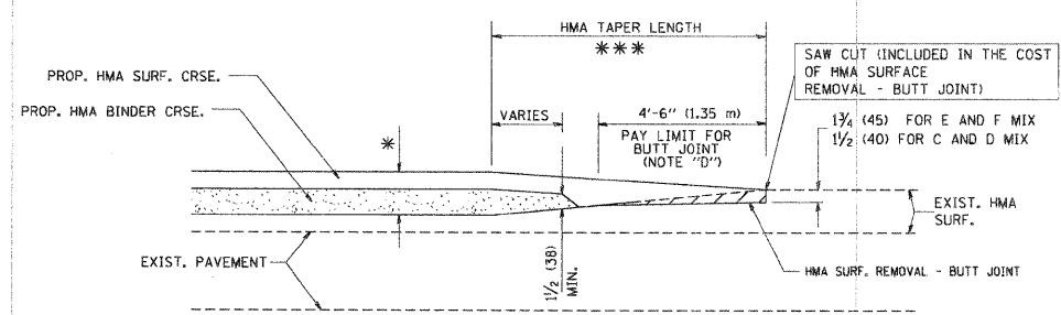
BUTT JOINT AND HMA TAPER
