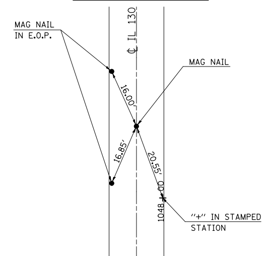
P.I. #40 STATION 1107+93.58 /57.75' LT.
