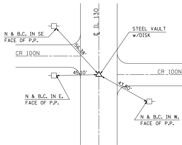
P.I. #5 STATION 1053+01.67 /0.49' RT.
