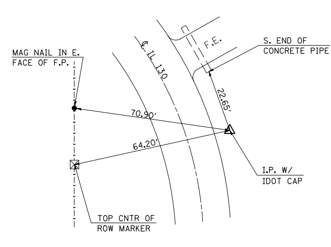
P.I. #111 STATION 1123+03.67 /23.89' RT.
