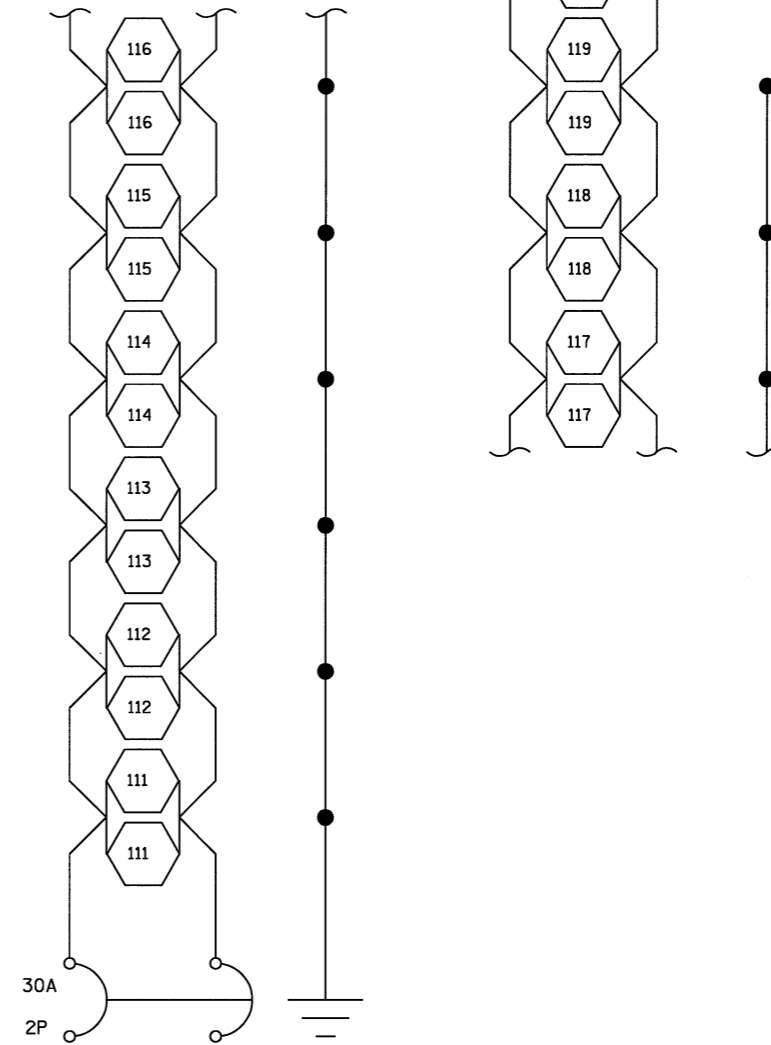
CIRCUIT #2 CONTROLLER #124
