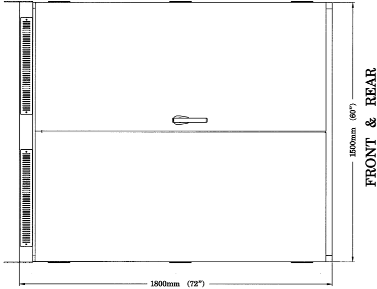
TUNNEL LIGHTING CONTROL SYSTEM CABINET EXTERIOR DETAIL
