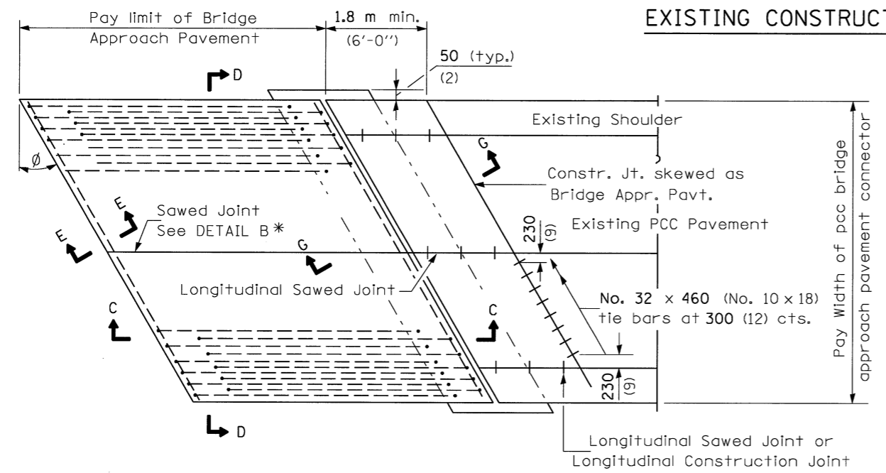
BRIDGE APPROACH PAVEMENT CONNECTOR (PCC)
