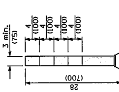
FLEXIBLE DELINEATOR
