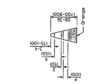
REFLECTORIZED CONE
