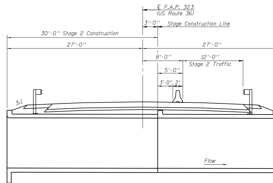
STAGE 2 CONSTRUCTION (Looking East)
