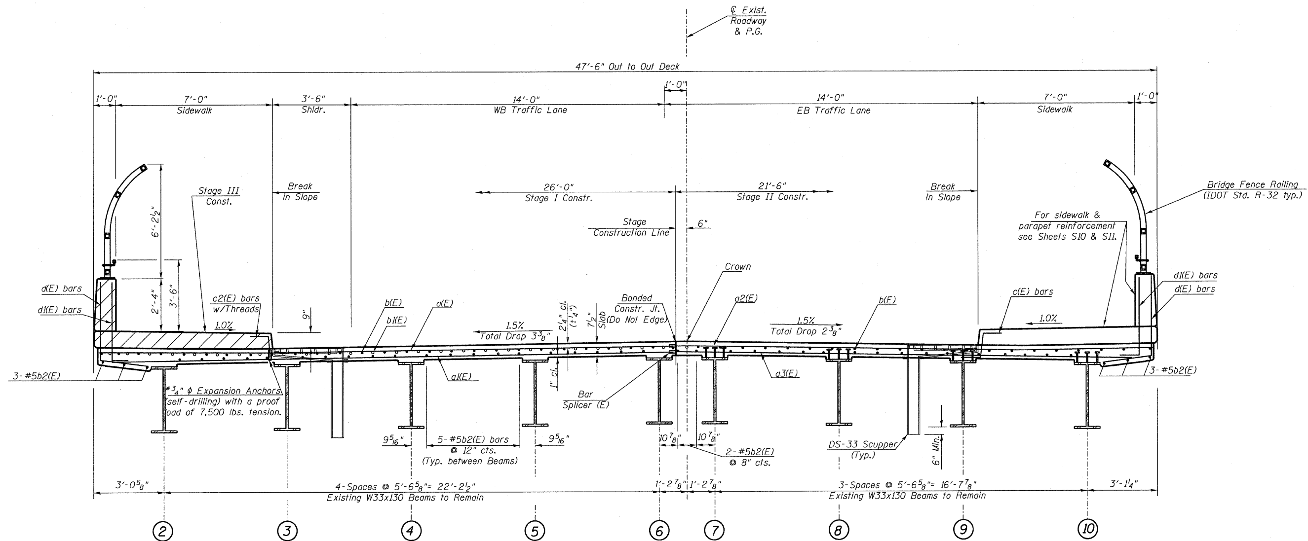
PROPOSED CROSS SECTION (Looking East)
